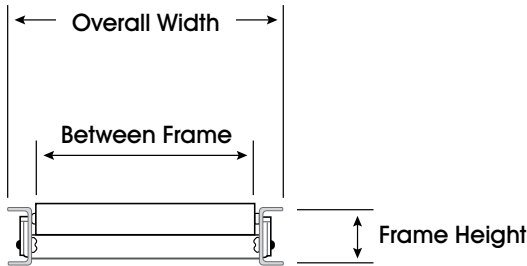
END VIEW
