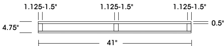
END VIEW
