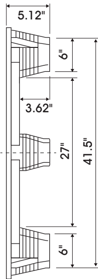
END VIEW
