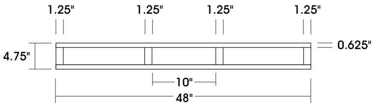
END VIEW
